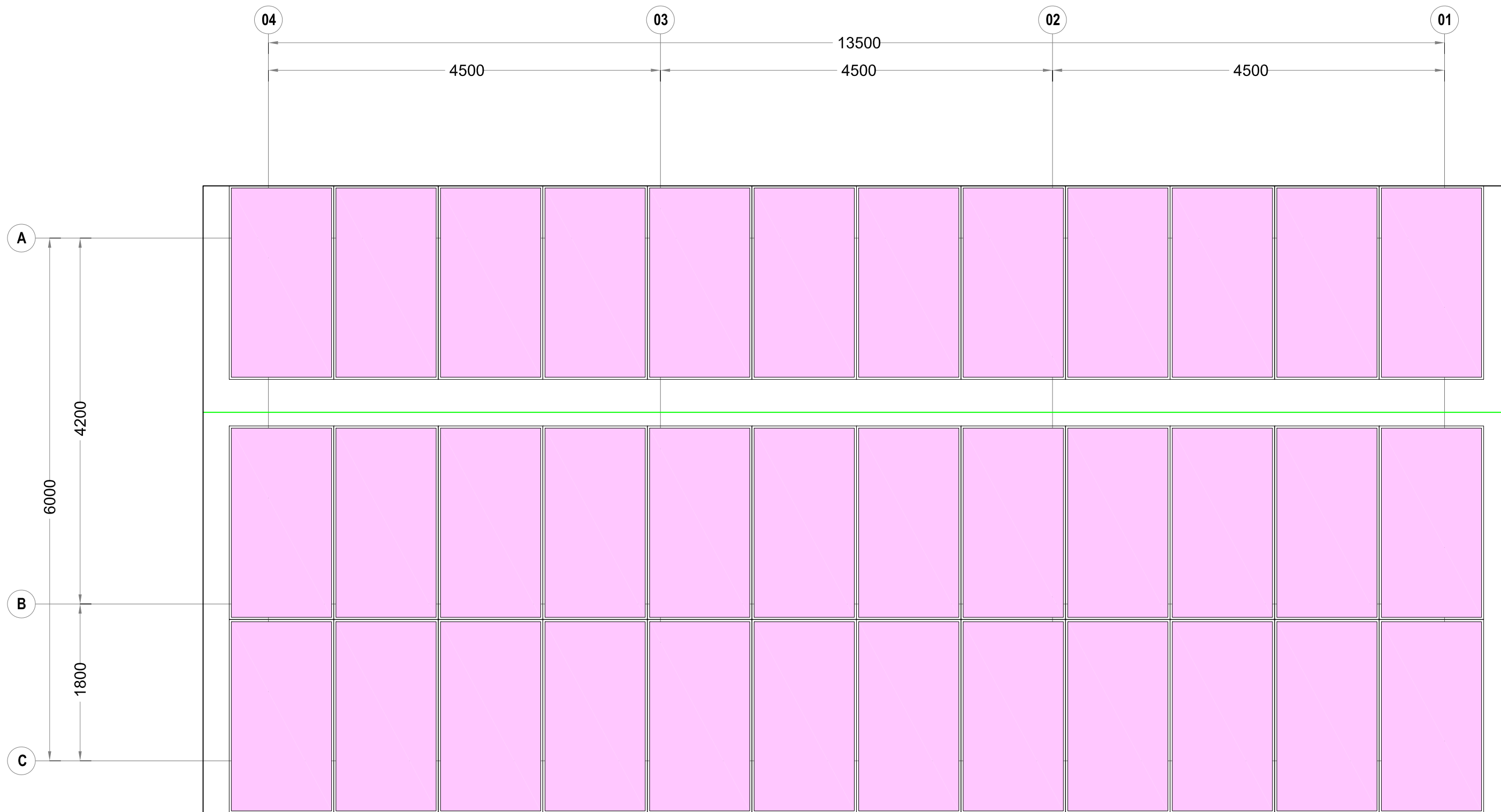
SOLAR PANELS ARRANGEMENT ON ROOF (MAXIMUM 36 Nos.)
