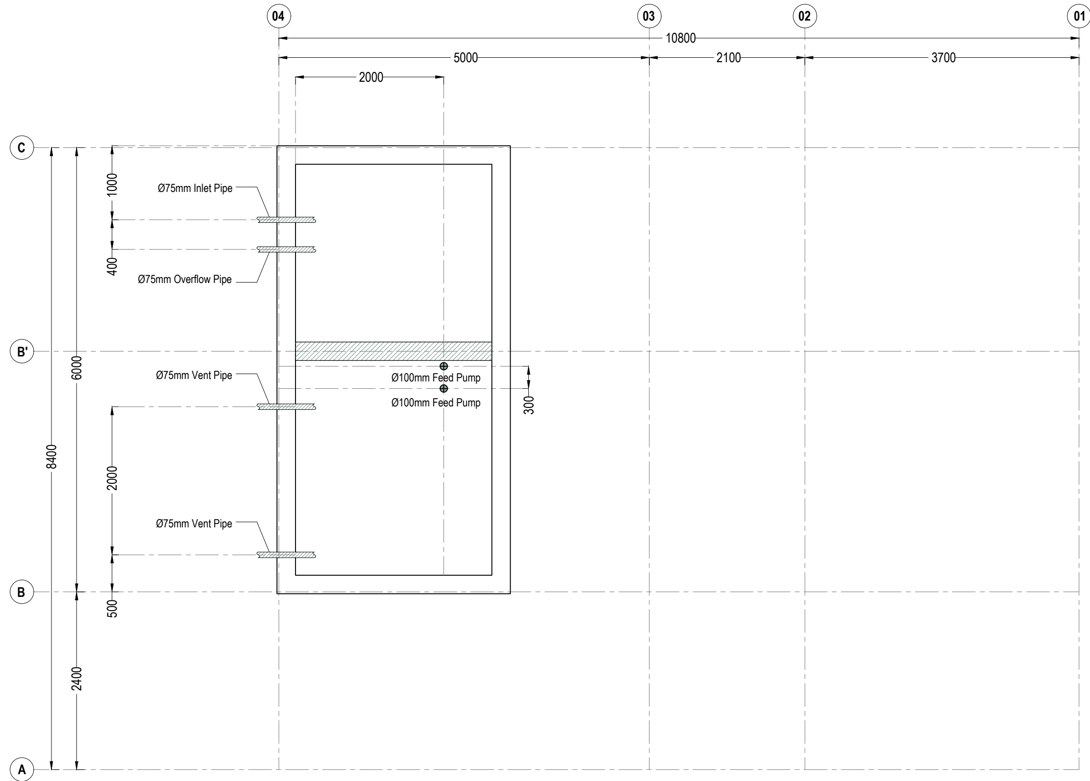
PIPE POSITION PLAN
