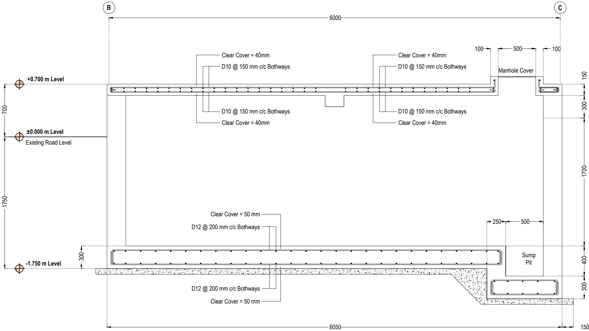
BASE SLAB & TOP SLAB SECTION (1-1)
