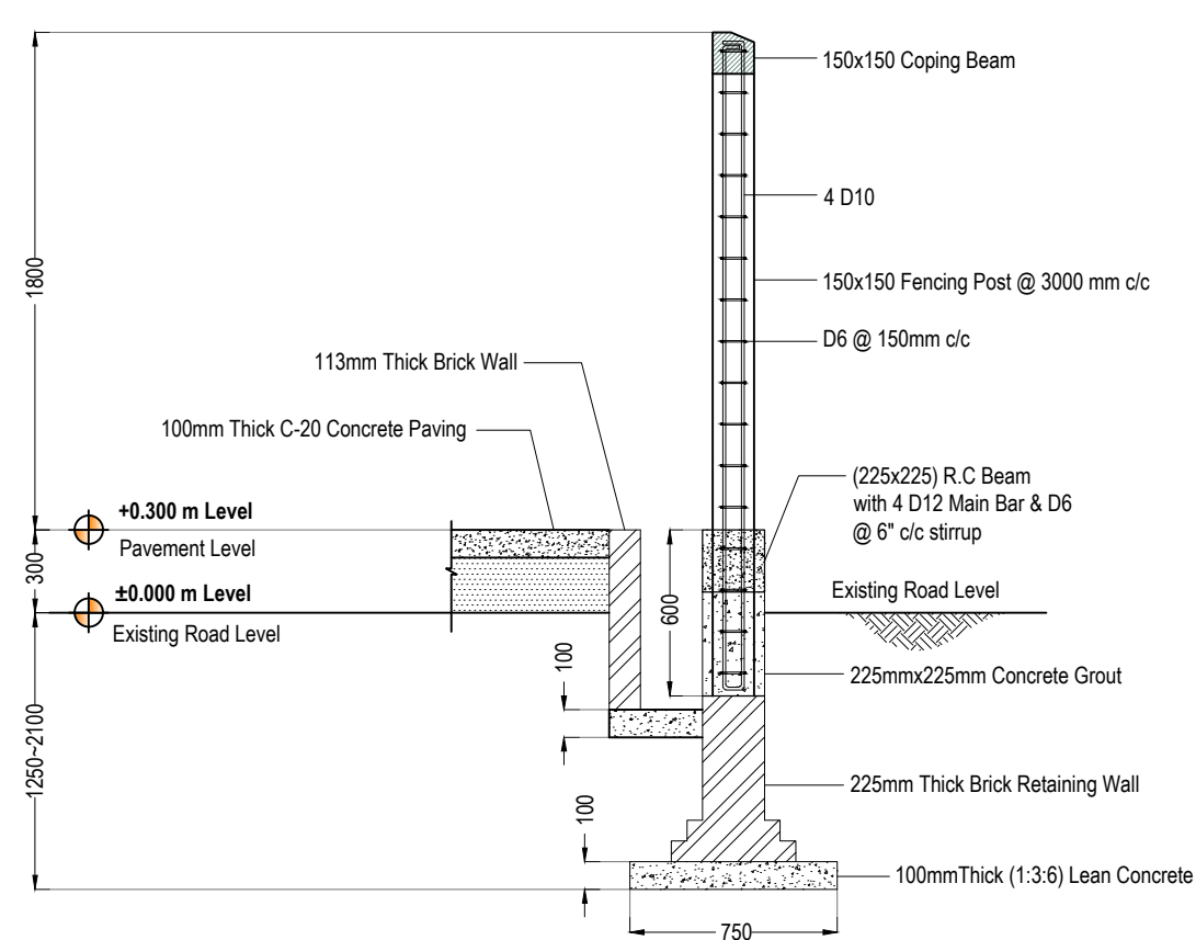
FENCING POST SECTION
