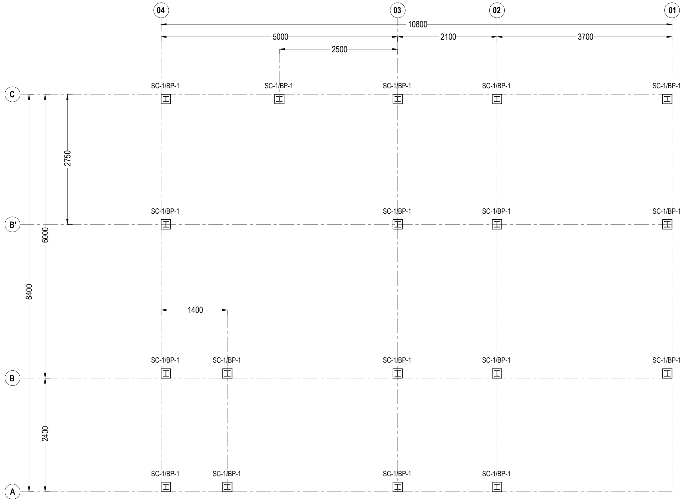
STEEL COLUMN & BASE PLATE PLAN (+0.700 m LEVEL TO +4.050m LEVEL)
