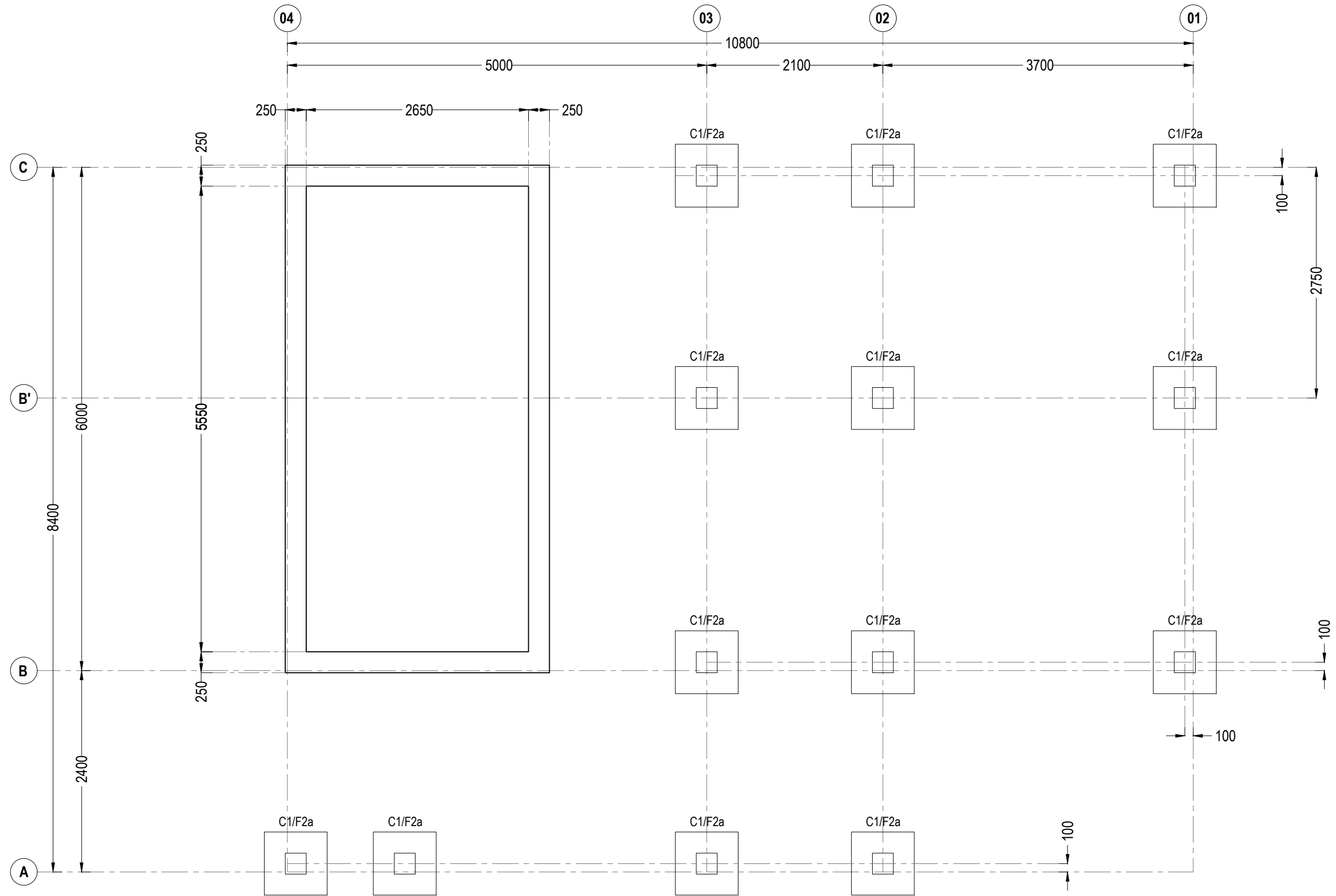
FOOTING PLAN
