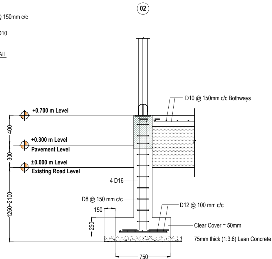
TYPICAL FOOTING SECTION (F2a)
