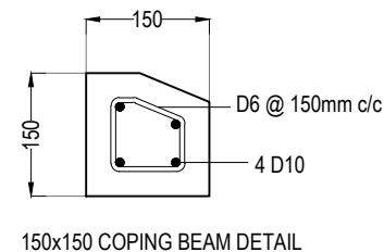
150x150 COPING BEAM DETAIL
