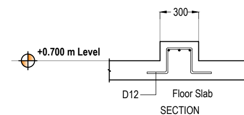
Floor Slab SECTION
