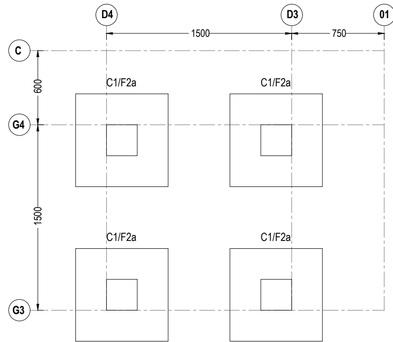
FOUNDATION PLAN (W.C) (-1.000m LEVEL)
