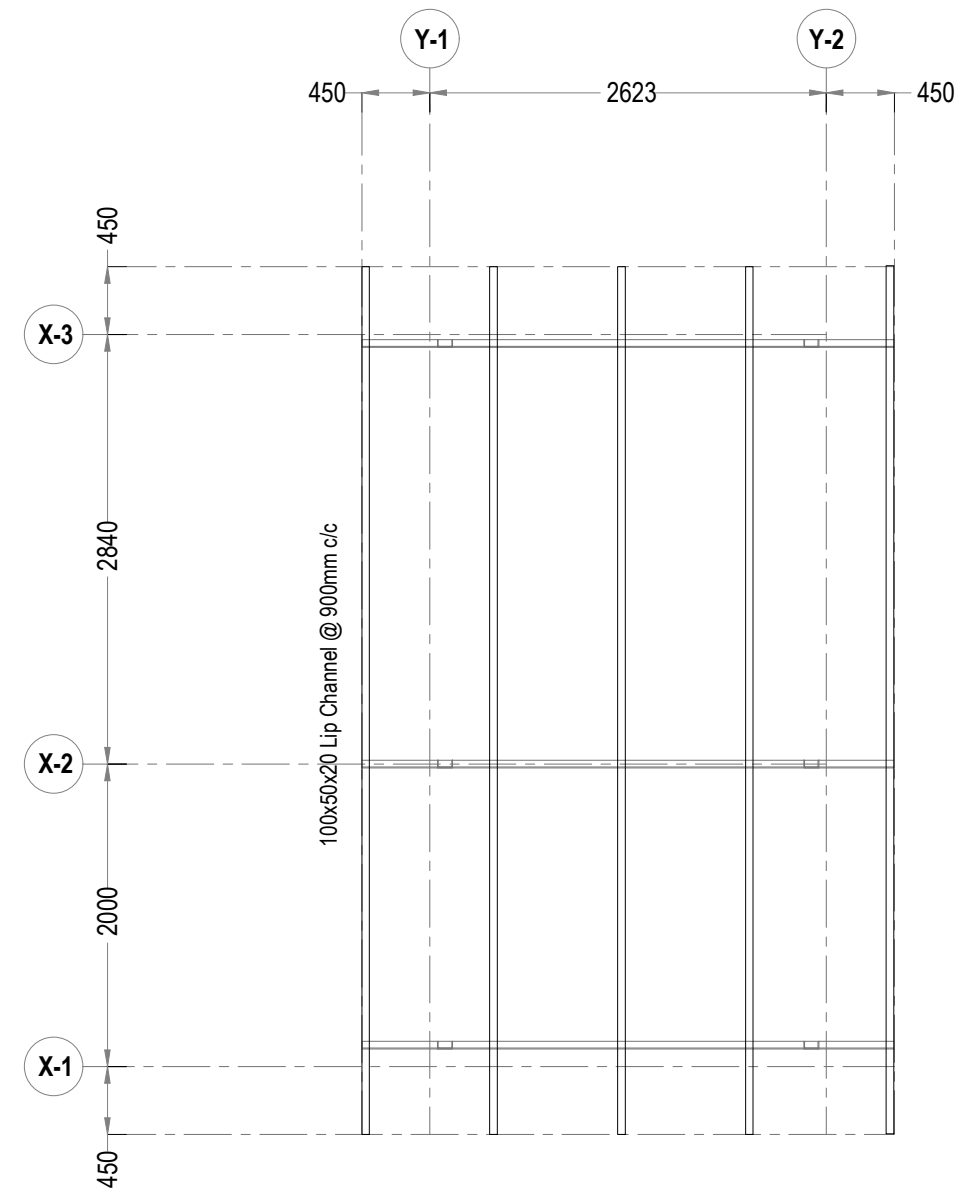
PURLIN PLAN
