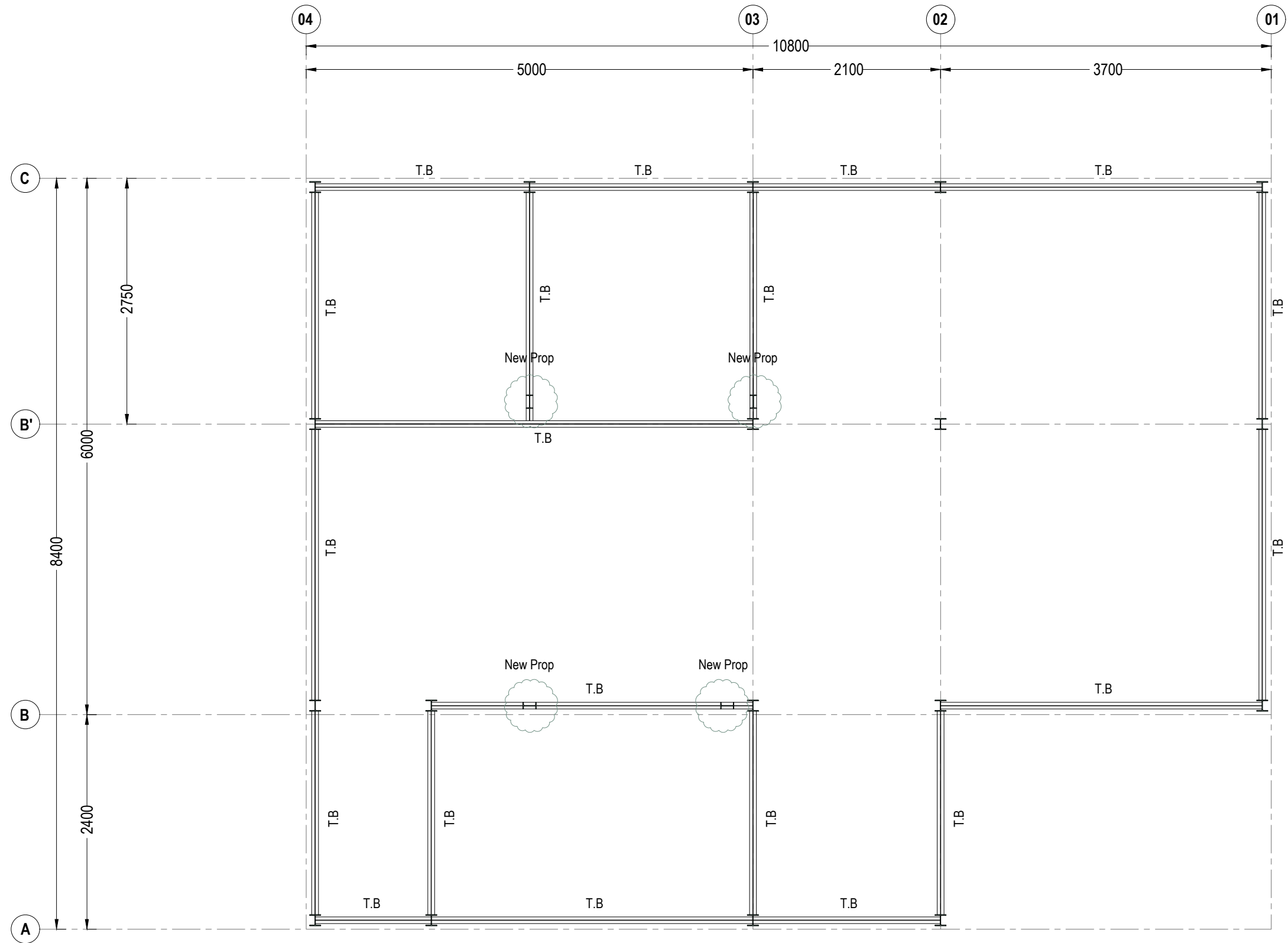
TIE BEAM PLAN (+4.050m LEVEL)
