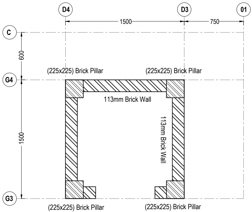
BRICK WALL PLAN (W.C)
