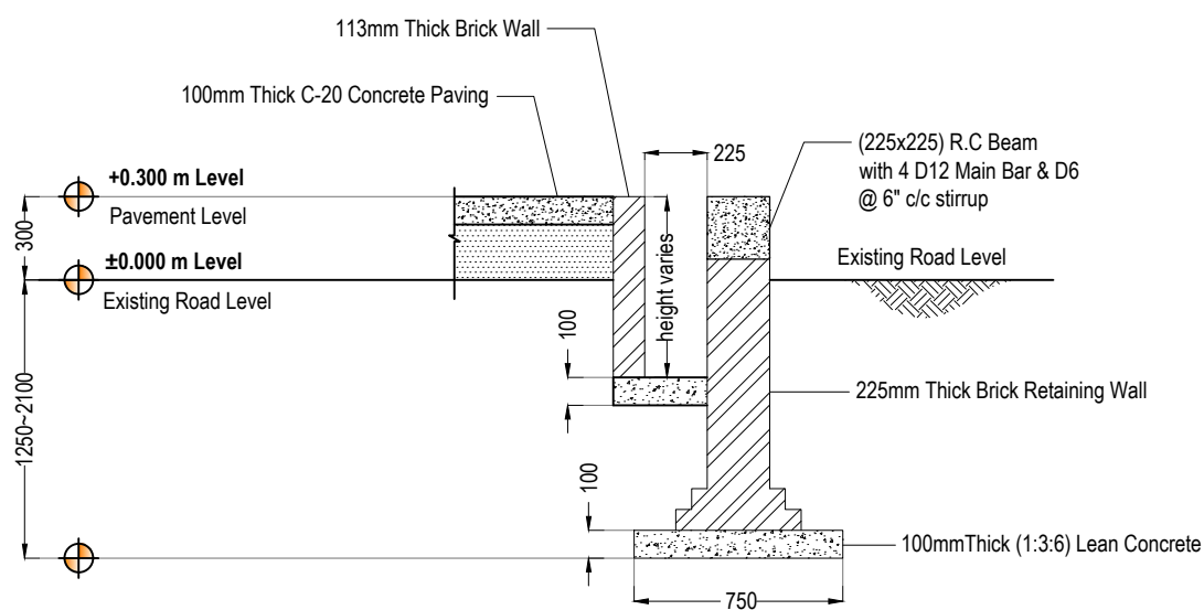
RETAINING WALL SECTION (A-A)
