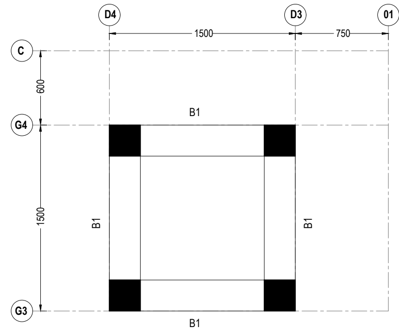
PLINTH BEAM PLAN (W.C) (+0.400m LEVEL)
