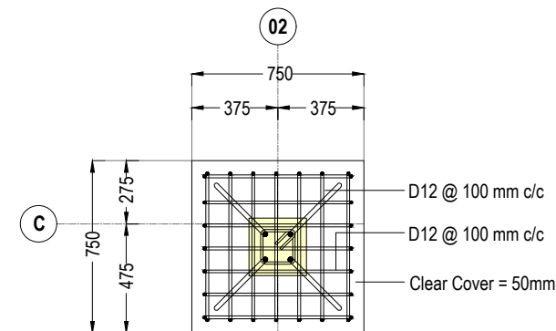
TYPICAL FOOTING REBAR ARRANGEMENT PLAN (F2a)
