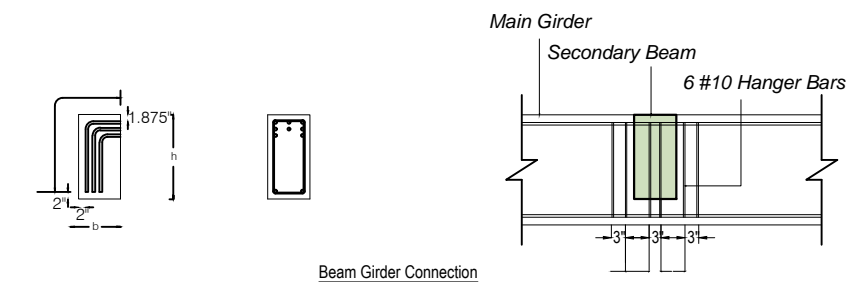
(C)Maximum Anchorage Length That can be Accommodated in a Given Primary (Girder) Section
