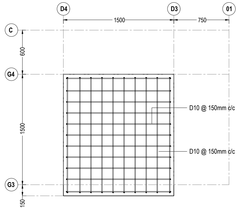
150mm THICK R.C TOP SLAB PLAN (W.C) (+3.000 m LEVEL)
