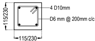
STIFFENER CROSS SECTION
