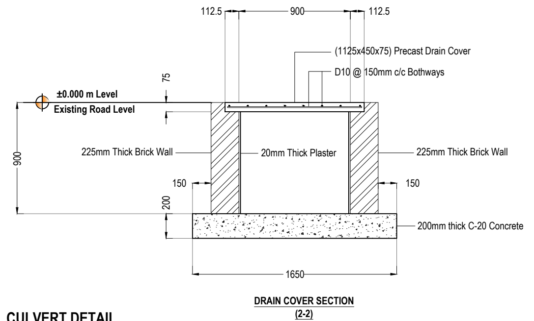
CULVERT DETAIL
