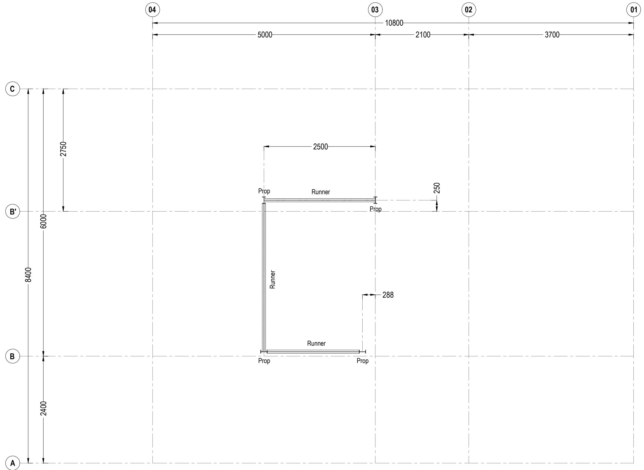
PROP & RUNNER PLAN
