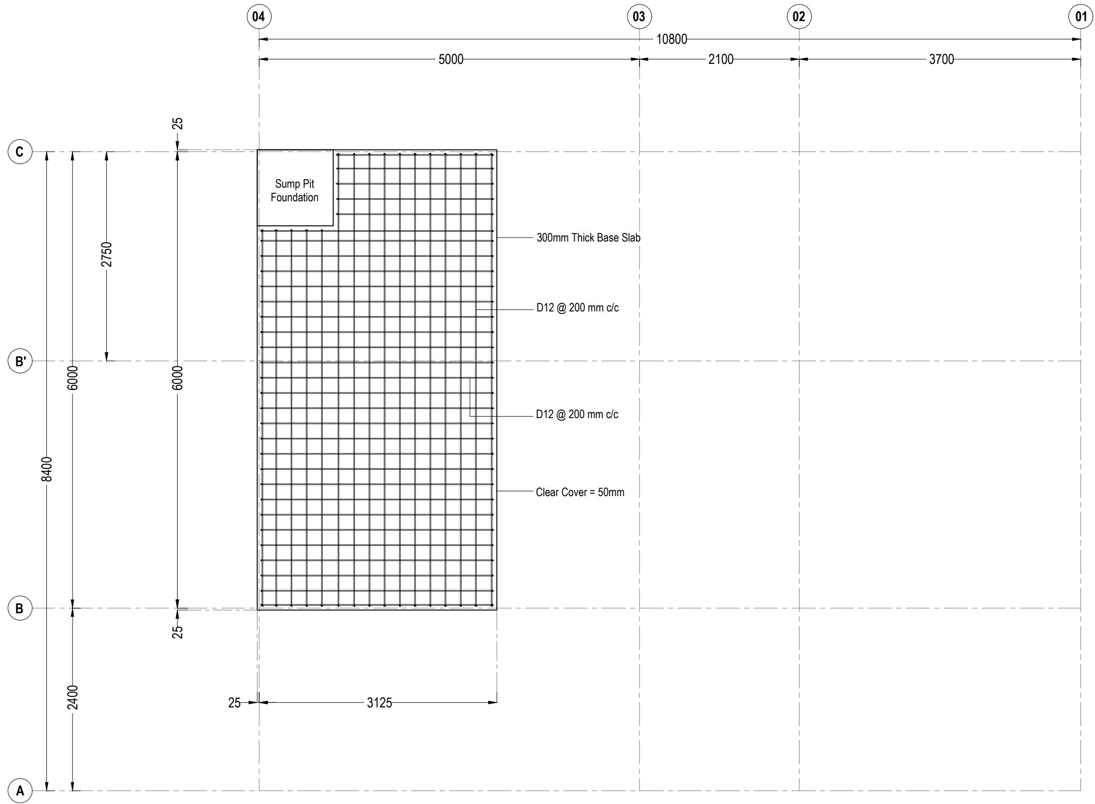
GROUND TANK BASE SLAB TOP & BOTTOM REBAR PLAN (-1.750 m LEVEL)
