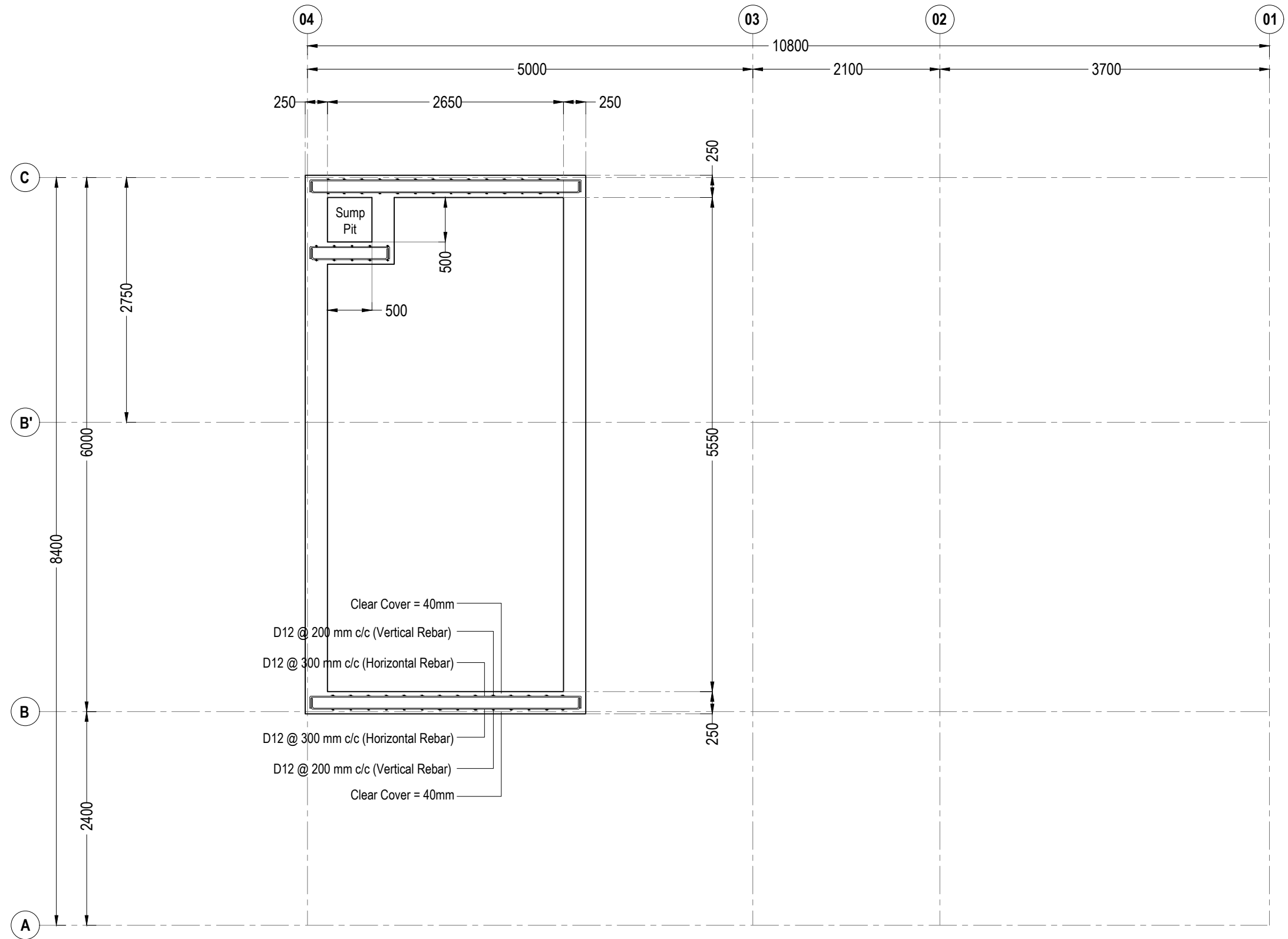
250mm THICK R.C WALL PLAN
